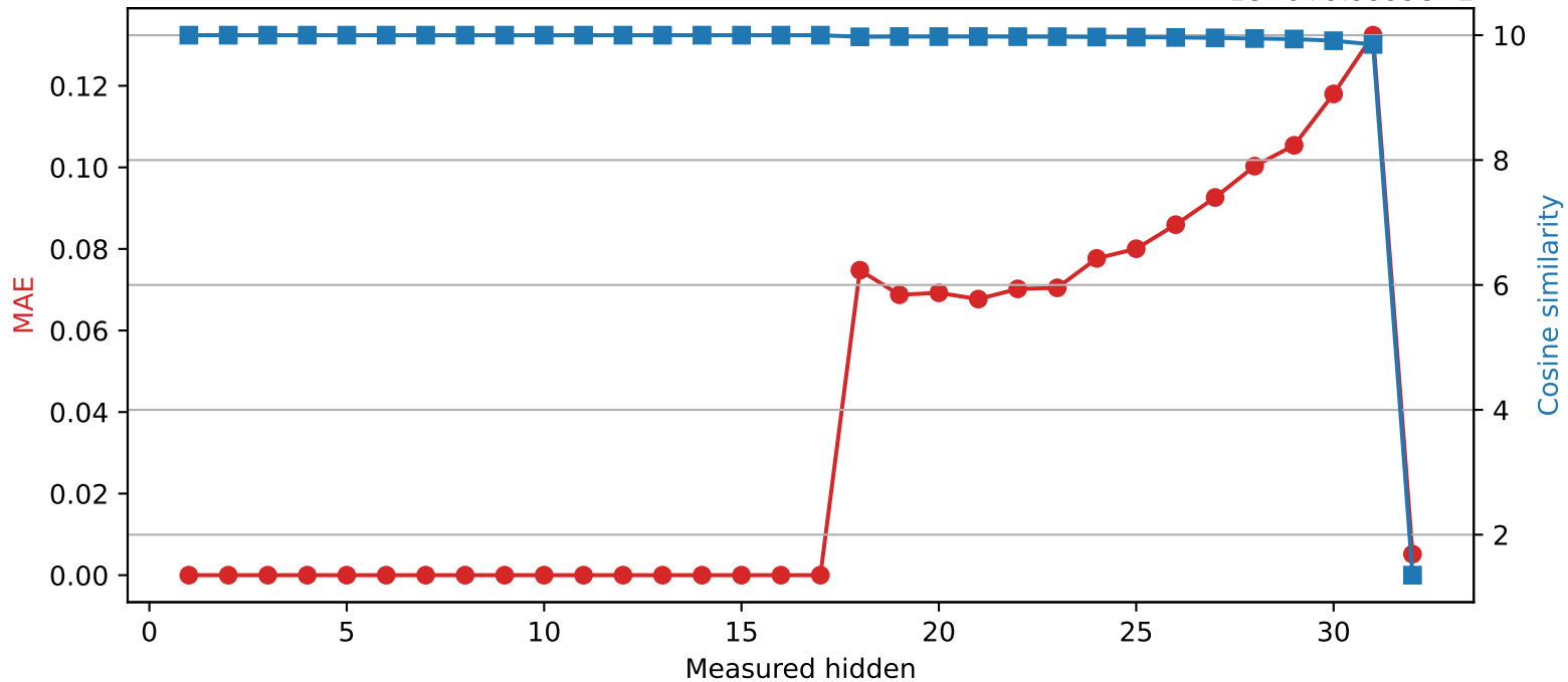
SmolLM2-360M | Quantized layer 17 | float64 → int8 1e-6+9.9999e-1
