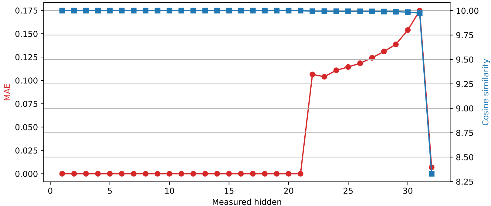
SmolLM2-360M | Quantized layer 21 | float64 → int8
