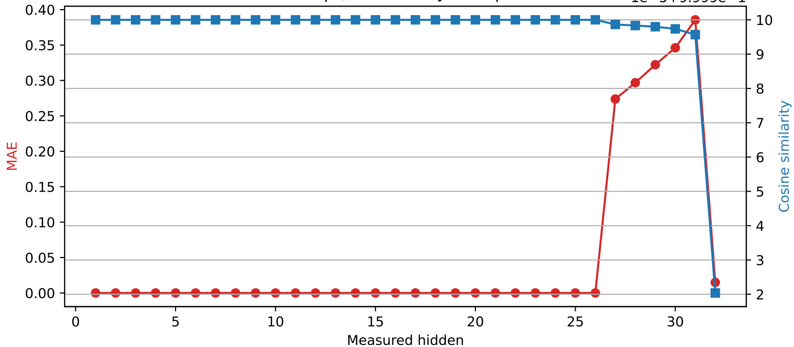
SmolLM2-360M | Quantized layer 26 | float64 → int8 1e-5 + 9.999e-1
