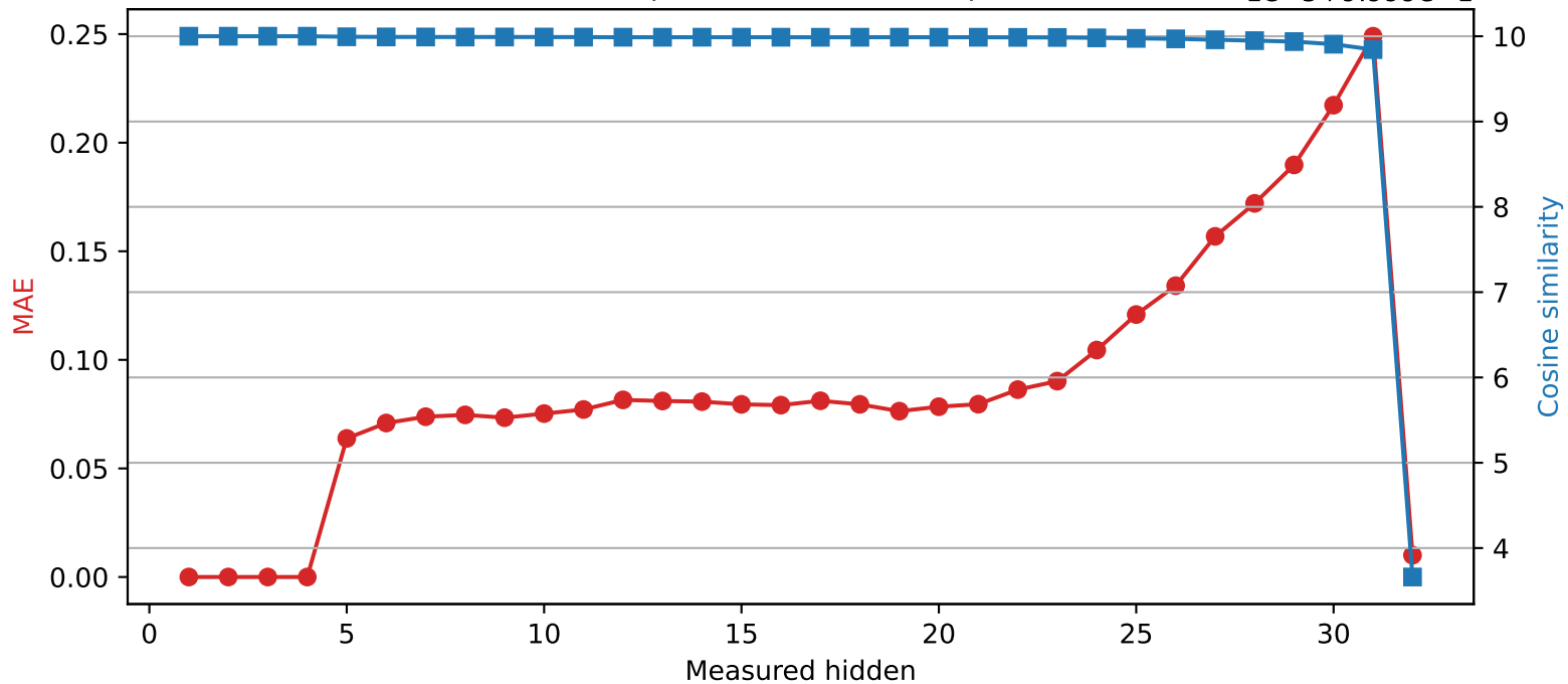
SmolLM2-360M | Quantized layer 4 | float64 → int8
