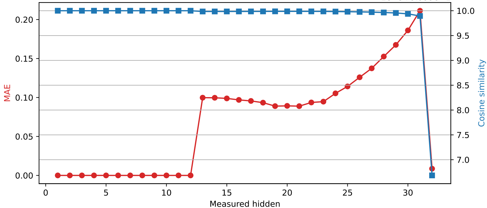
SmolLM2-360M | Quantized layer 12 | float64 → int8 1e-5 + 9.999e-1
