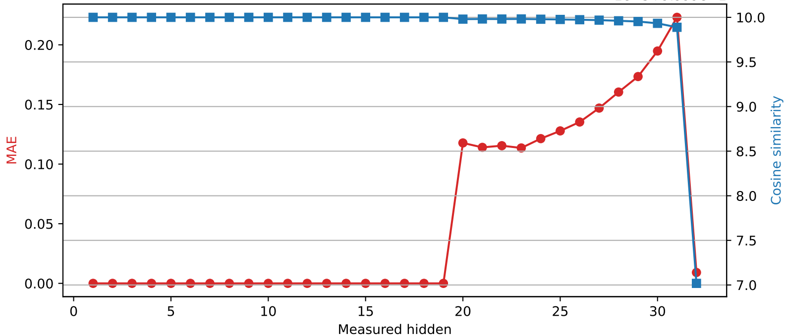
SmolLM2-360M | Quantized layer 19 | float64 → int8 1e-5+9.999e-1
