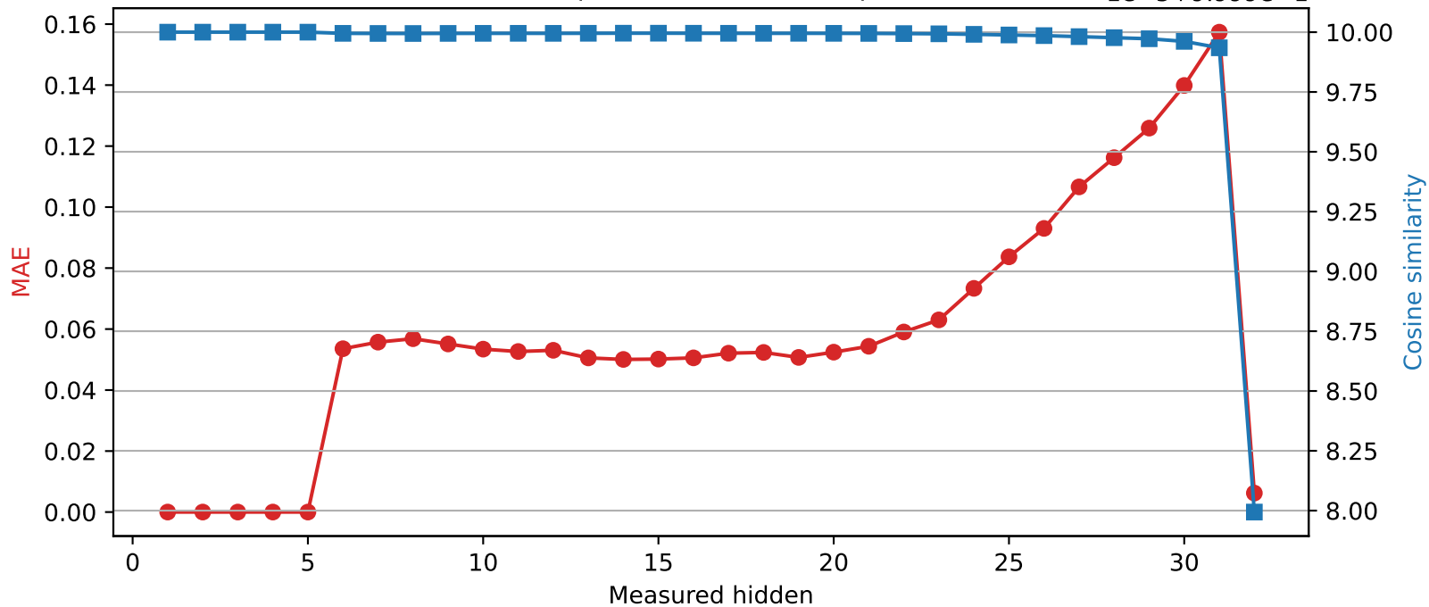
SmolLM2-360M | Quantized layer 5 | float64 → int8
