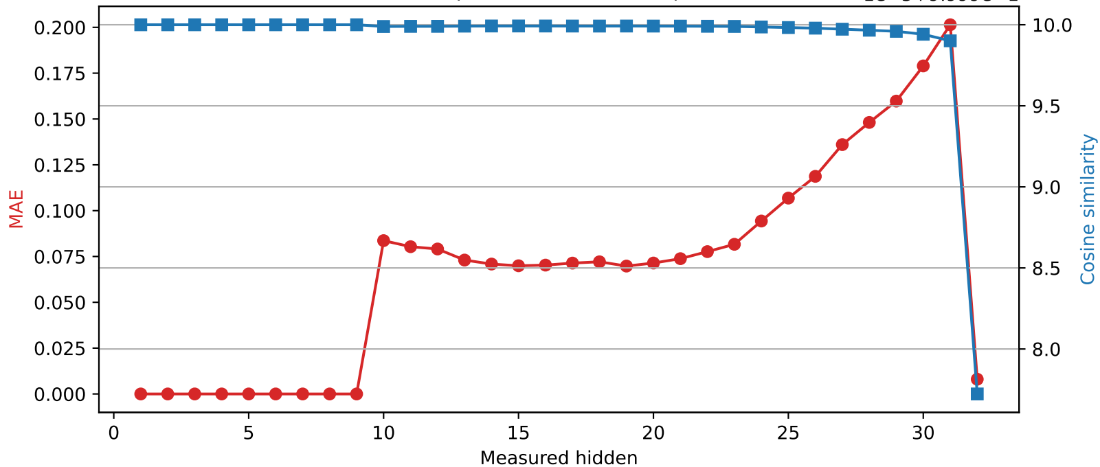
SmolLM2-360M | Quantized layer 9 | float64 → int8
