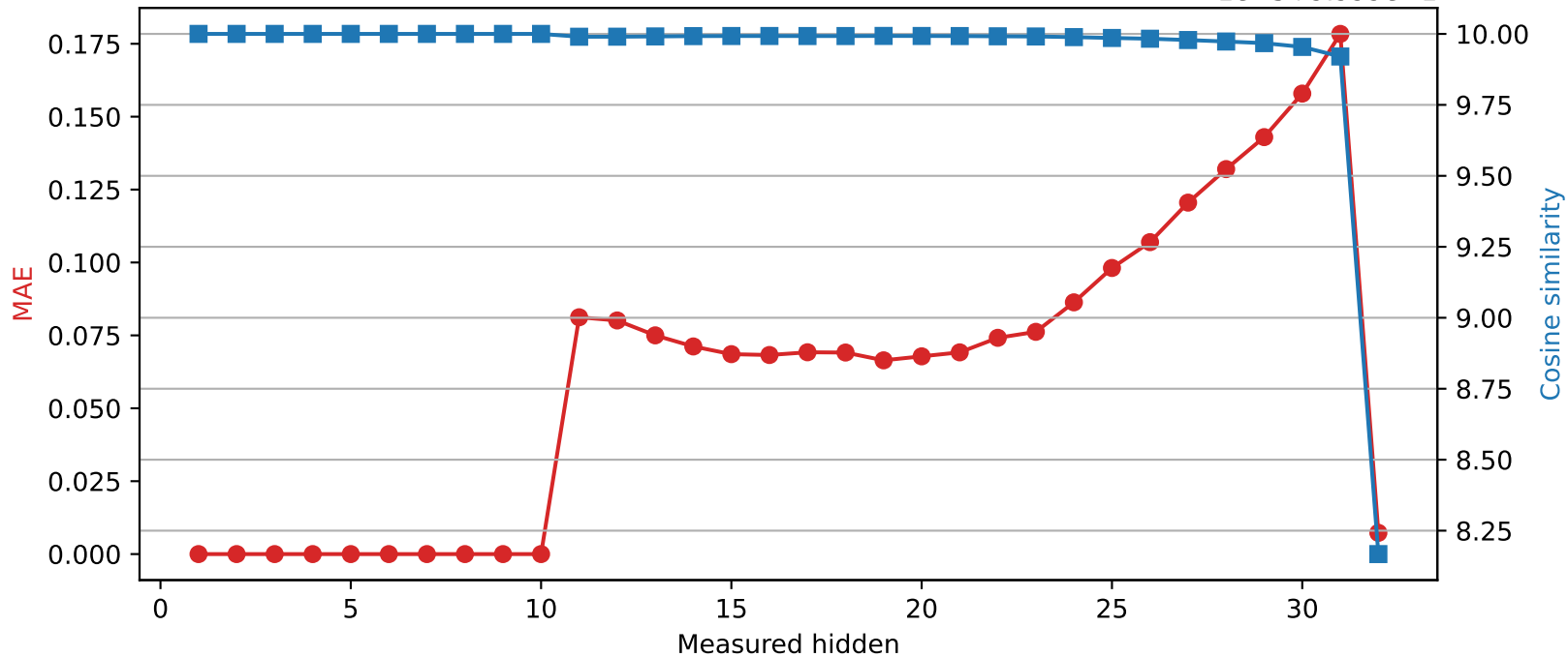
SmolLM2-360M | Quantized layer 10 | float64 → int8 1e-5 + 9.999e-1
