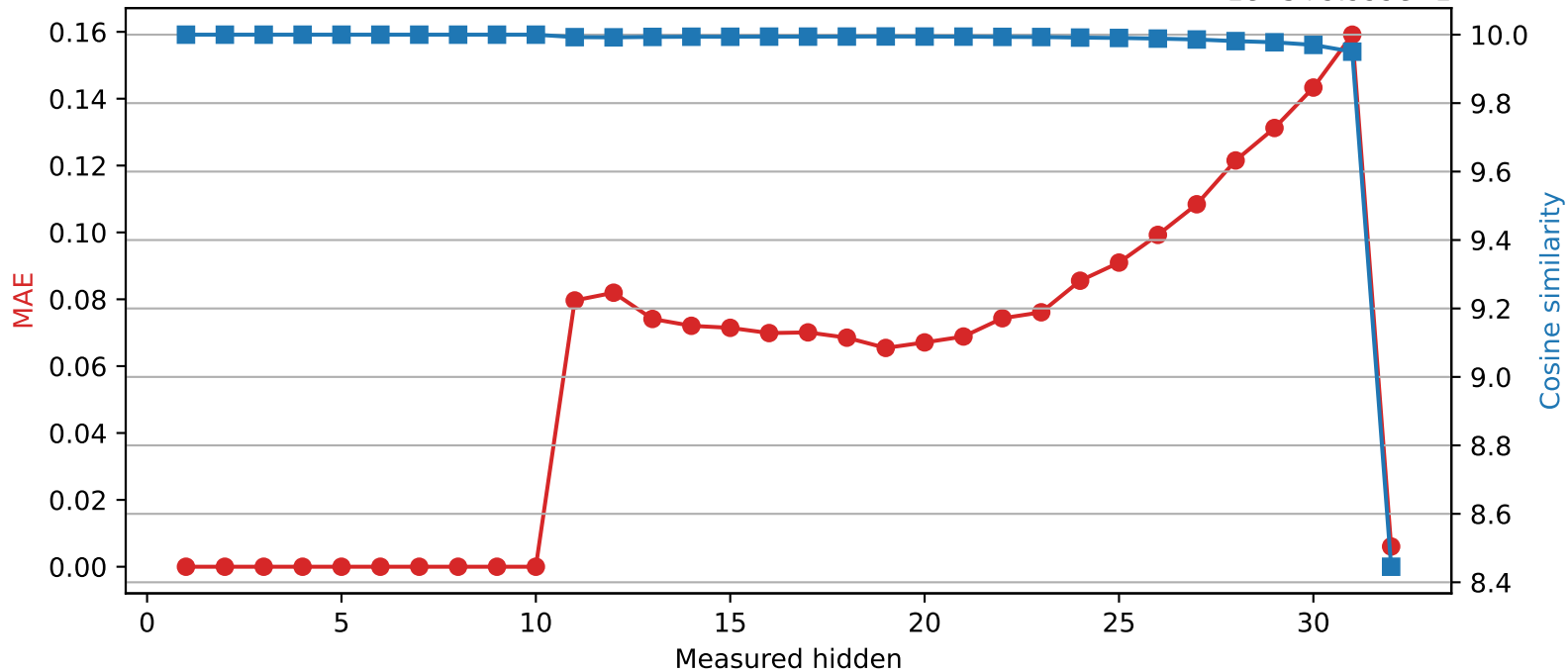
SmolLM2-360M | Quantized layer 10 | float64 → int8 1e-5+9.999e-1
