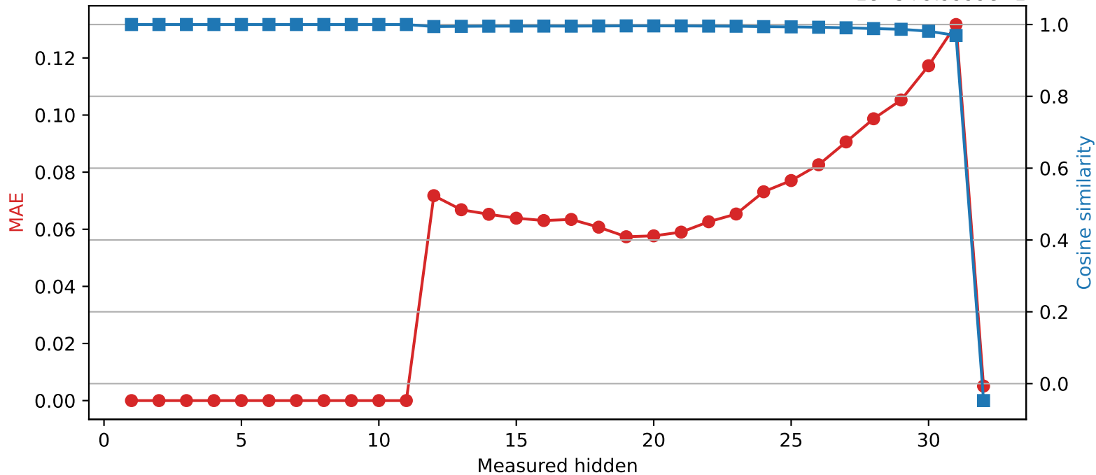
SmolLM2-360M | Quantized layer 11 | float64 → int8 1e-5 + 9.9999e-1
