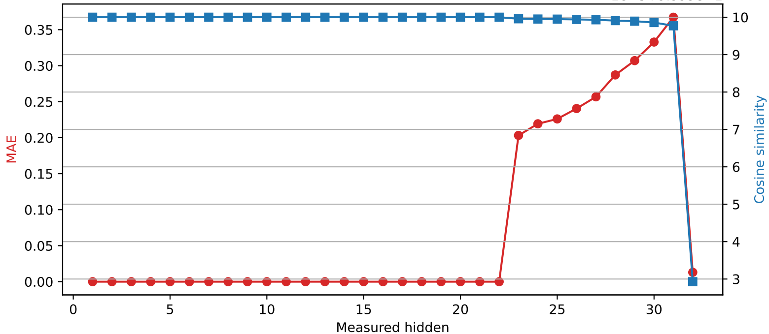
SmolLM2-360M | Quantized layer 22 | float64 → int8 1e-5+9.999e-1
