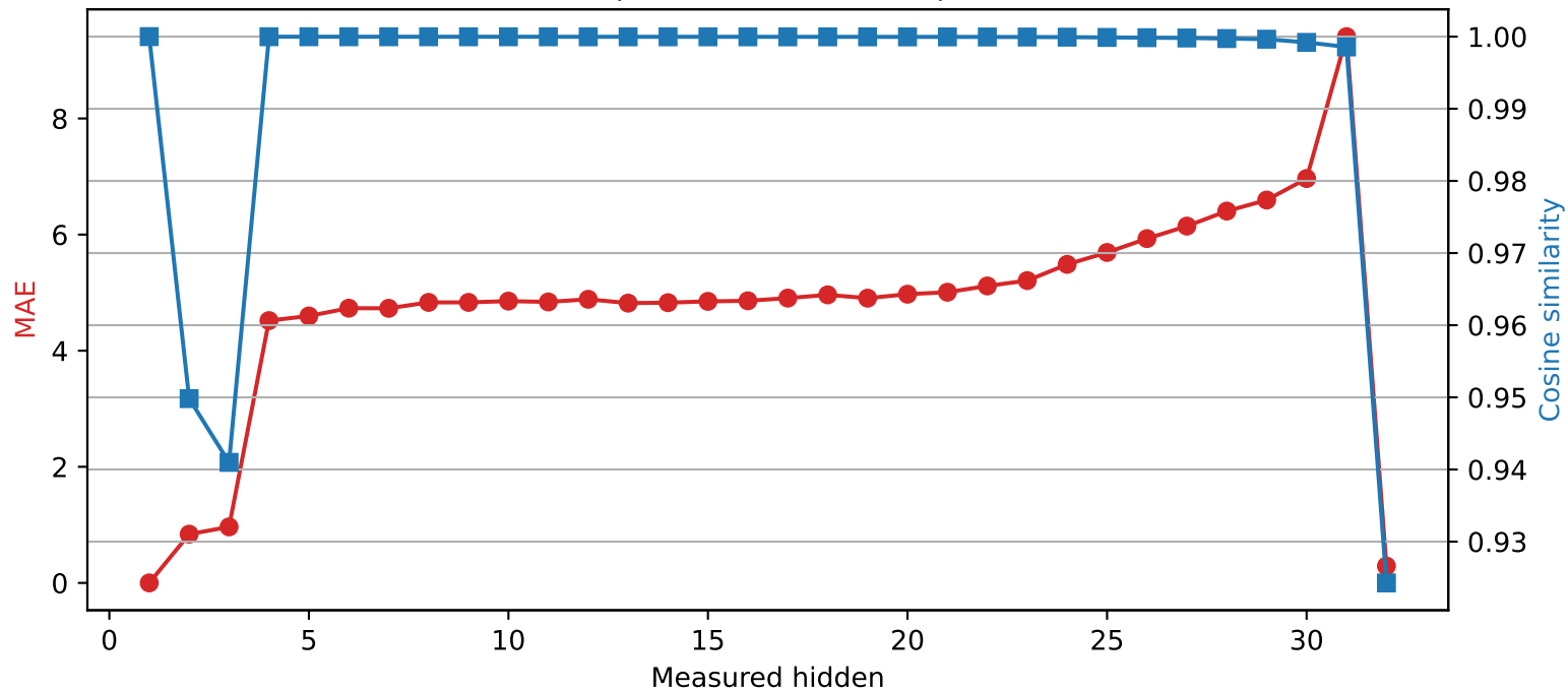
SmolLM2-360M | Quantized layer 1 | float16 \rightarrow int4
