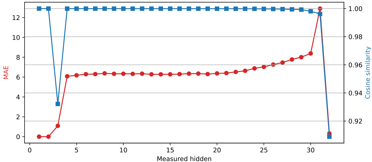
SmolLM2-360M | Quantized layer 2 | float16 → int4
