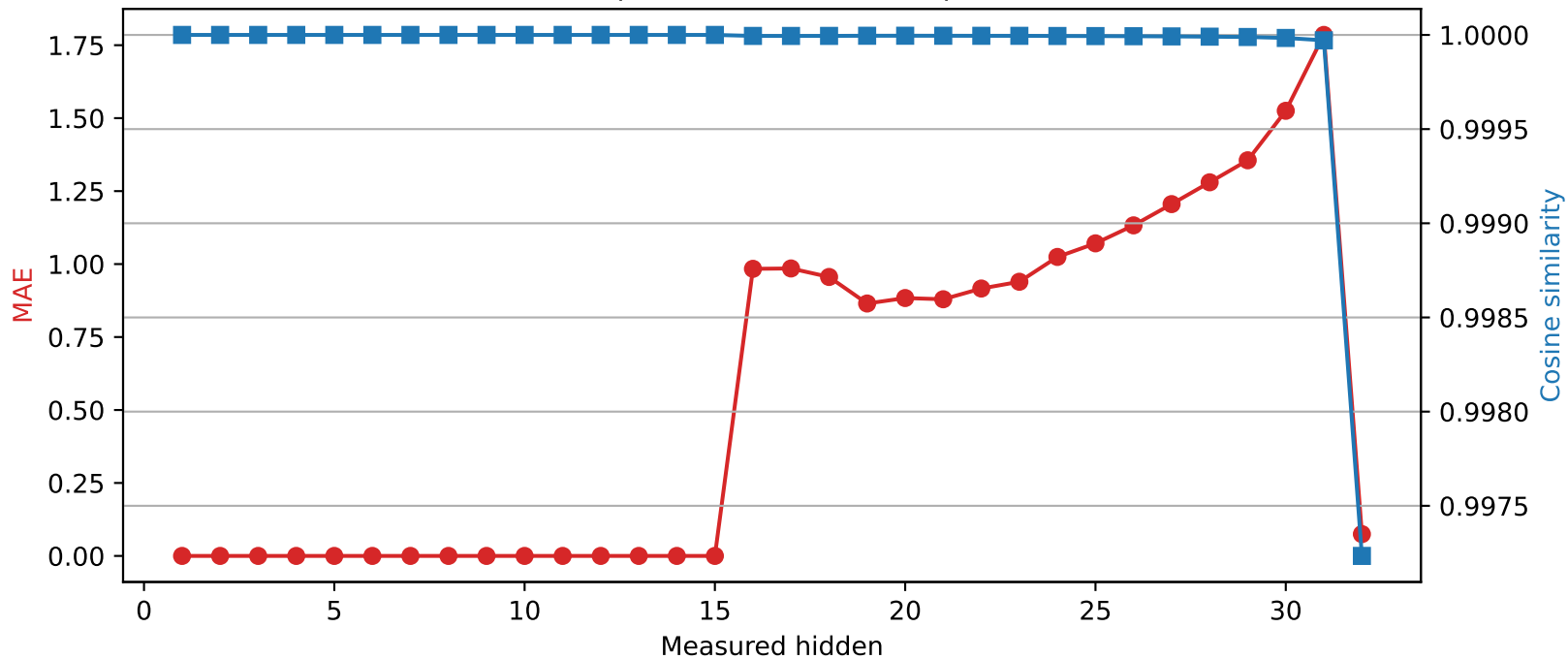
SmolLM2-360M | Quantized layer 15 | float16 \rightarrow int4
