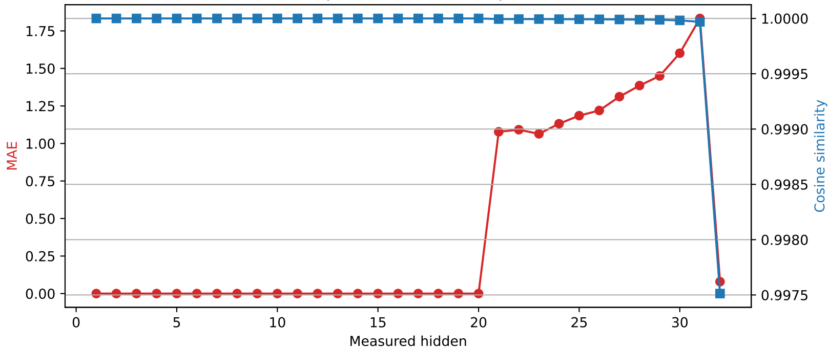
SmolLM2-360M | Quantized layer 20 | float16 → int4
