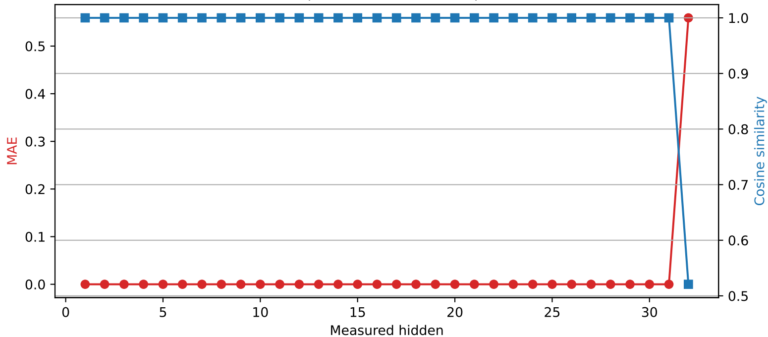
SmolLM2-360M | Quantized layer 31 | float16 → int4
