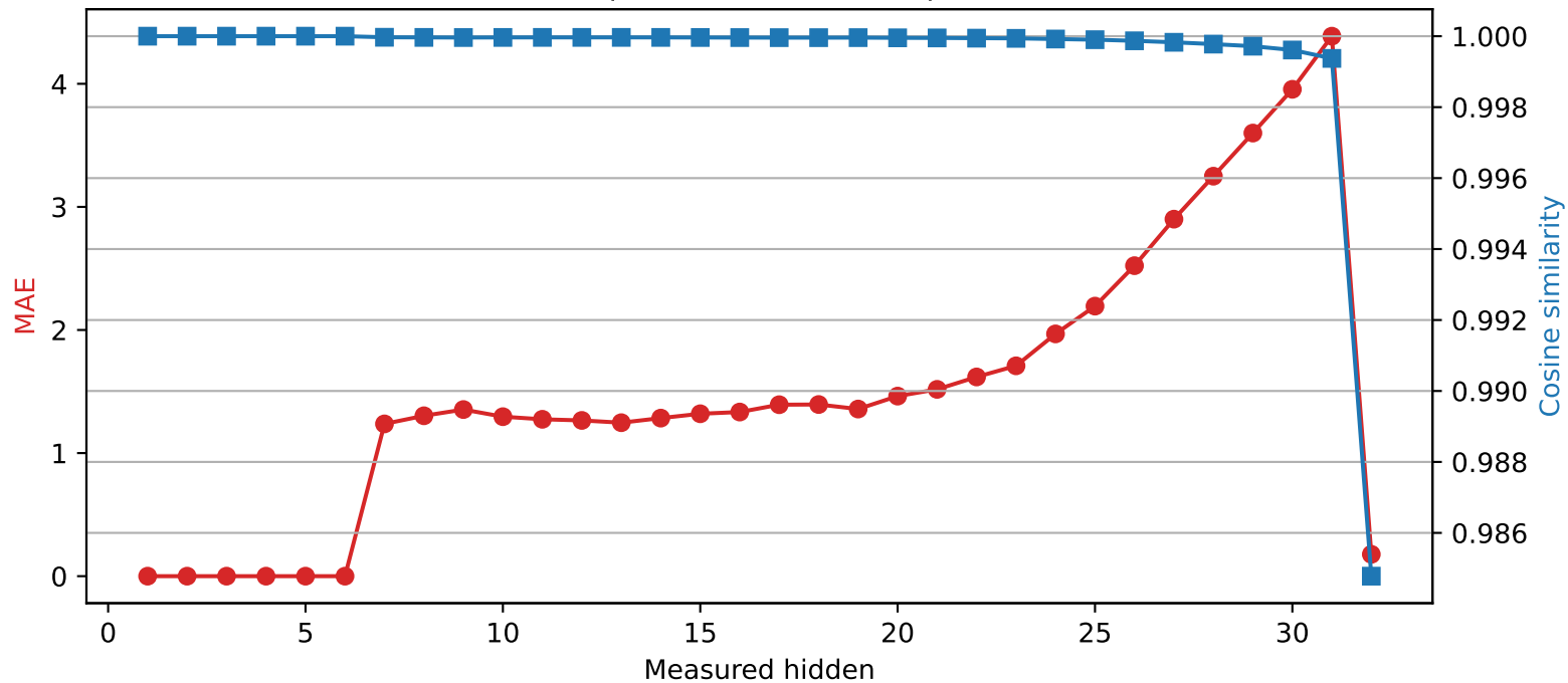
SmolLM2-360M | Quantized layer 6 | float16 \rightarrow int4
