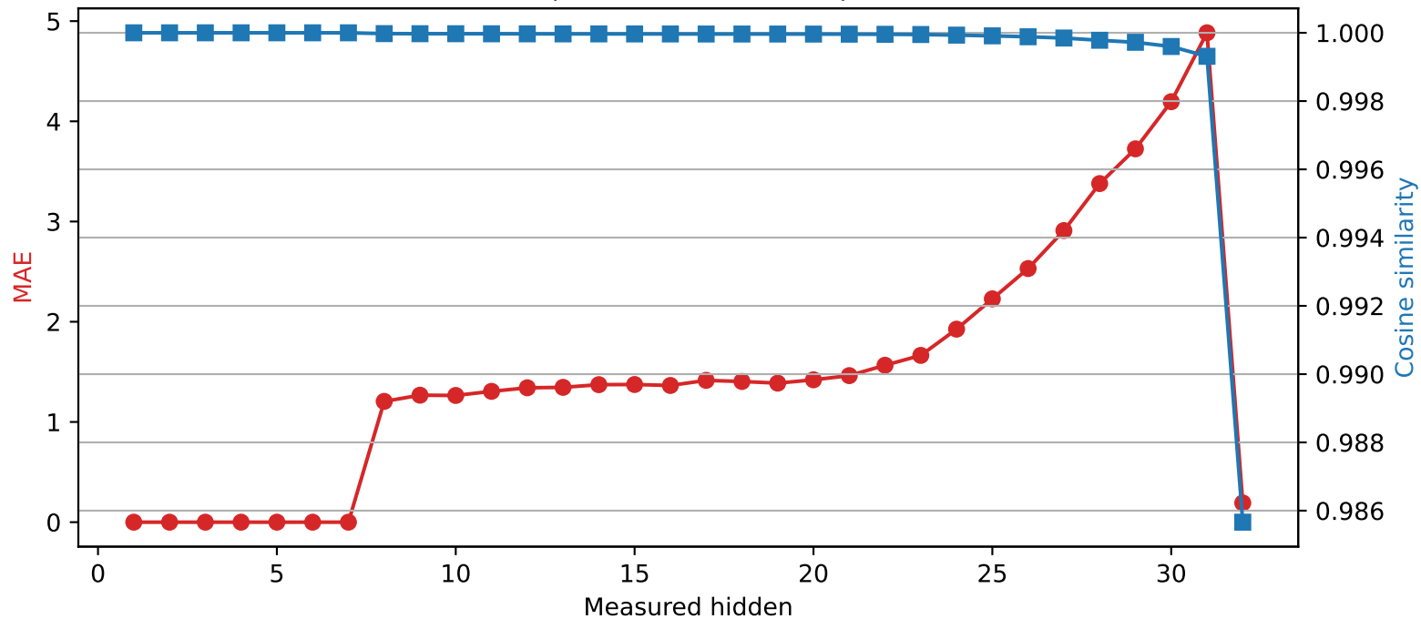
SmolLM2-360M | Quantized layer 7 | float16 \rightarrow int4
