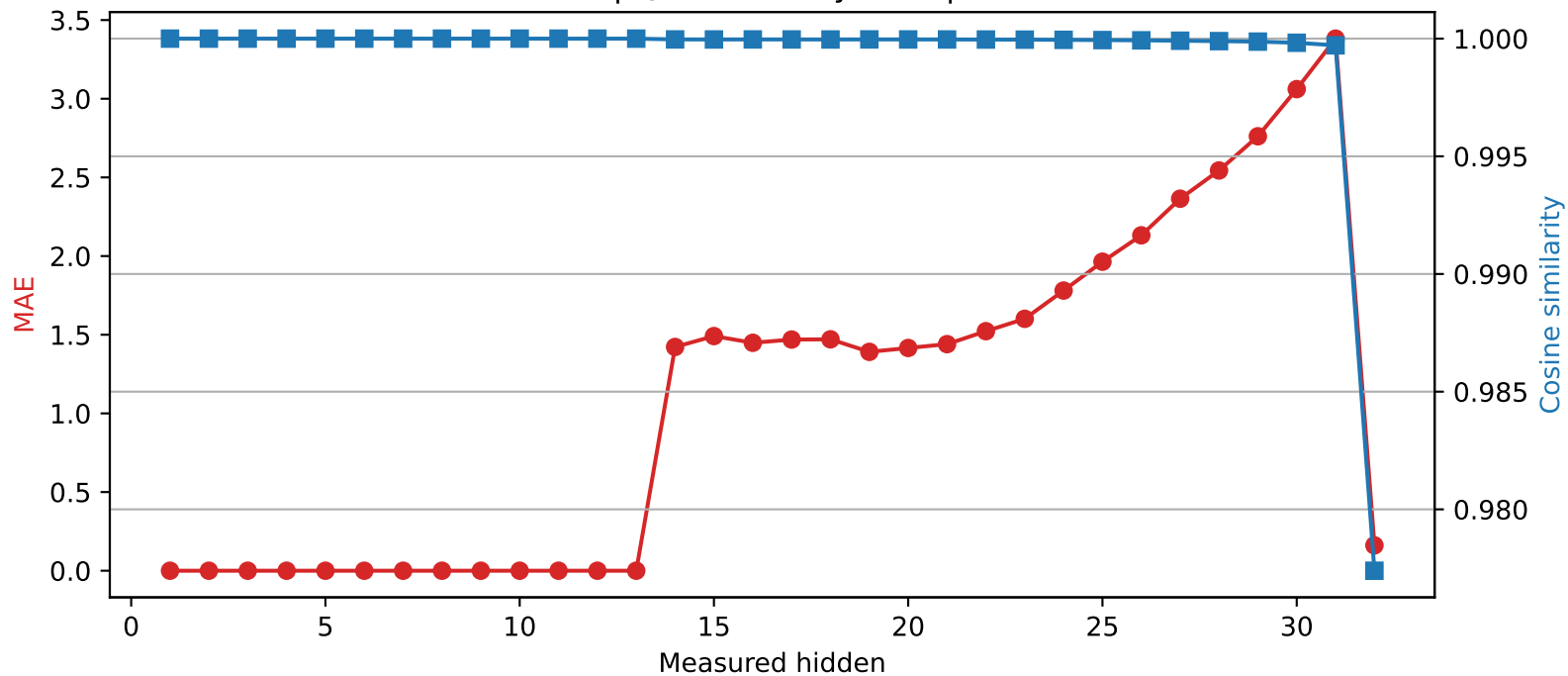
SmolLM2-360M | Quantized layer 13 | float16 \rightarrow int4
