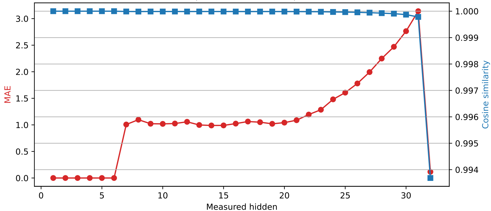
SmolLM2-360M | Quantized layer 6 | float16 → int4
