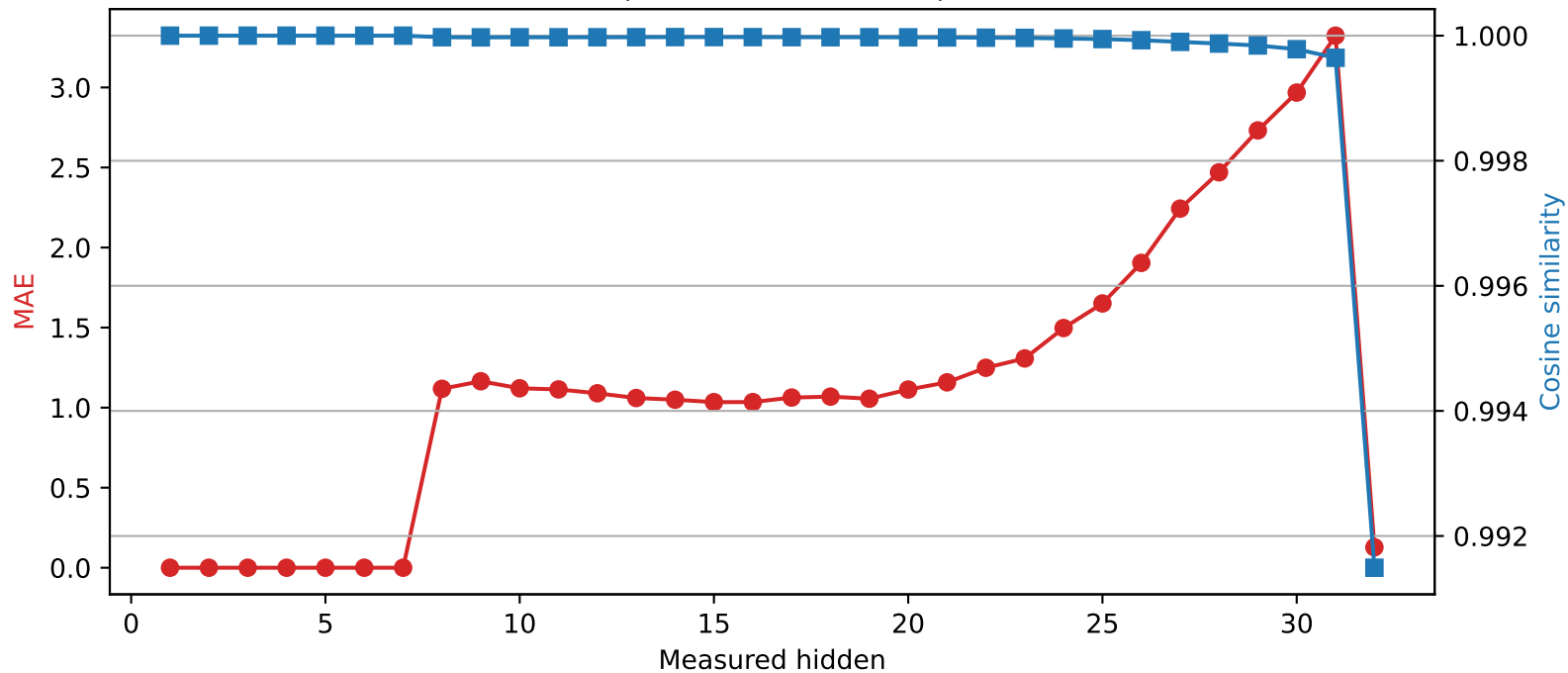
SmolLM2-360M | Quantized layer 7 | float32 → int4
