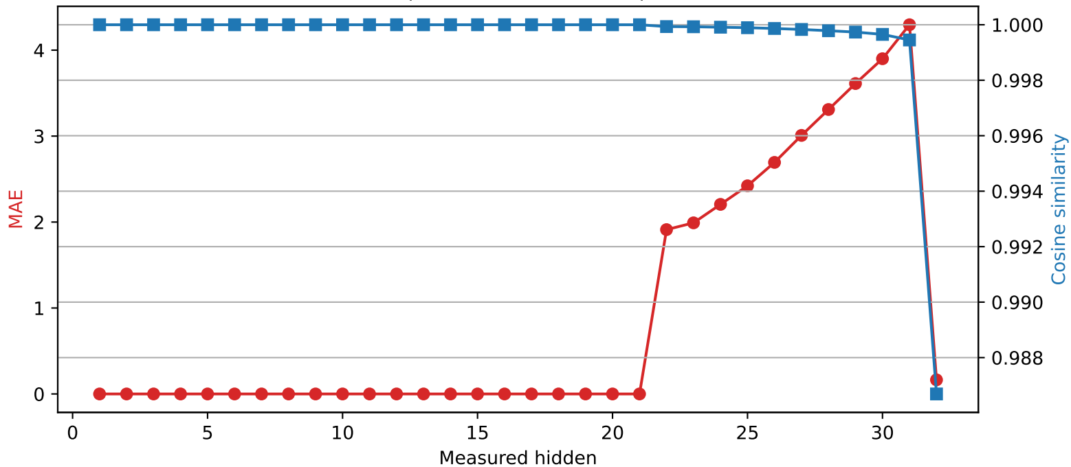
SmolLM2-360M | Quantized layer 21 | float32 → int4
