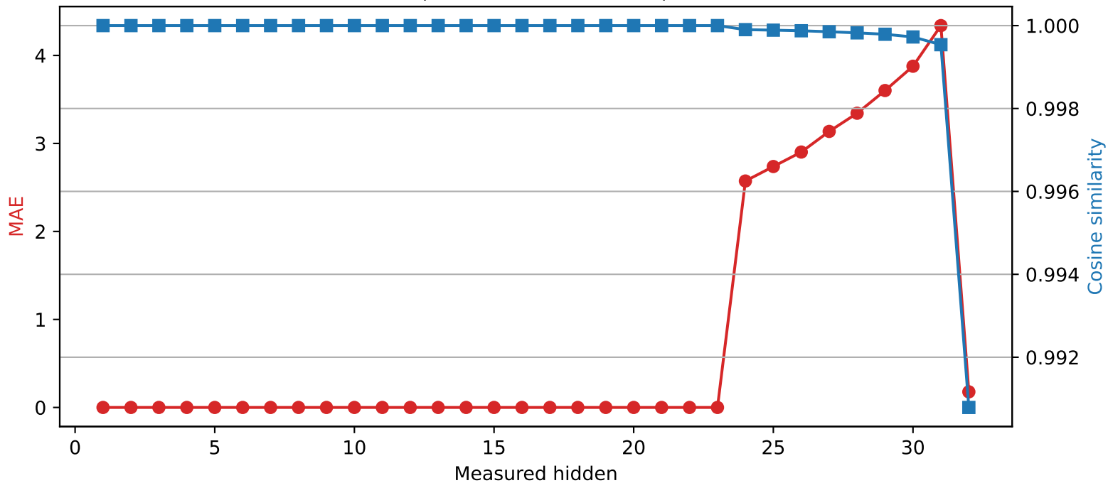
SmolLM2-360M | Quantized layer 23 | float32 → int4
