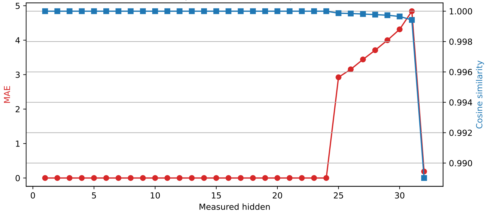
SmolLM2-360M | Quantized layer 24 | float32 → int4
