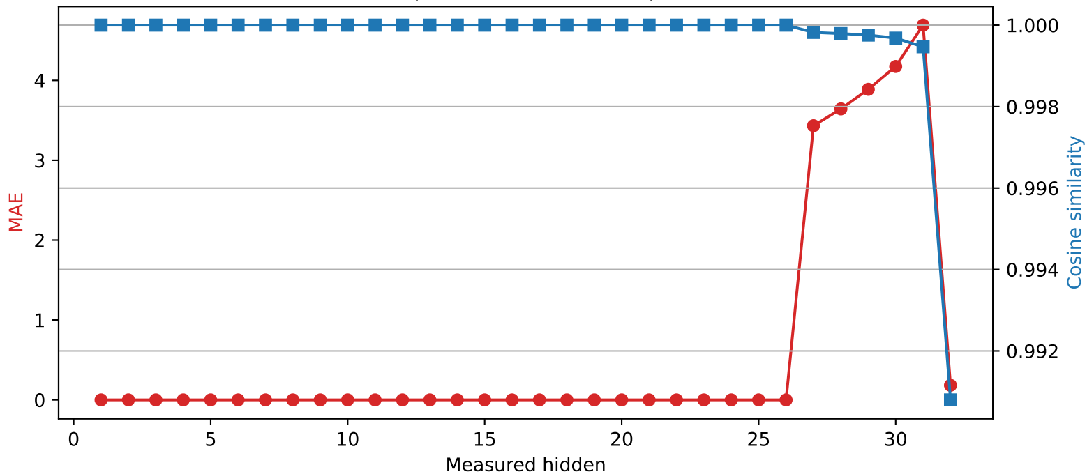
SmolLM2-360M | Quantized layer 26 | float32 → int4
