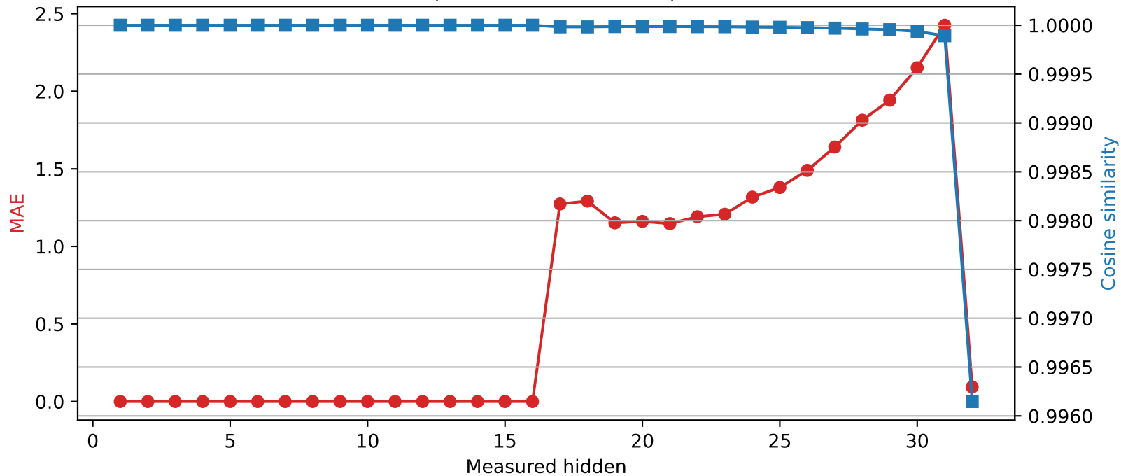
SmolLM2-360M | Quantized layer 16 | float32 → int4
