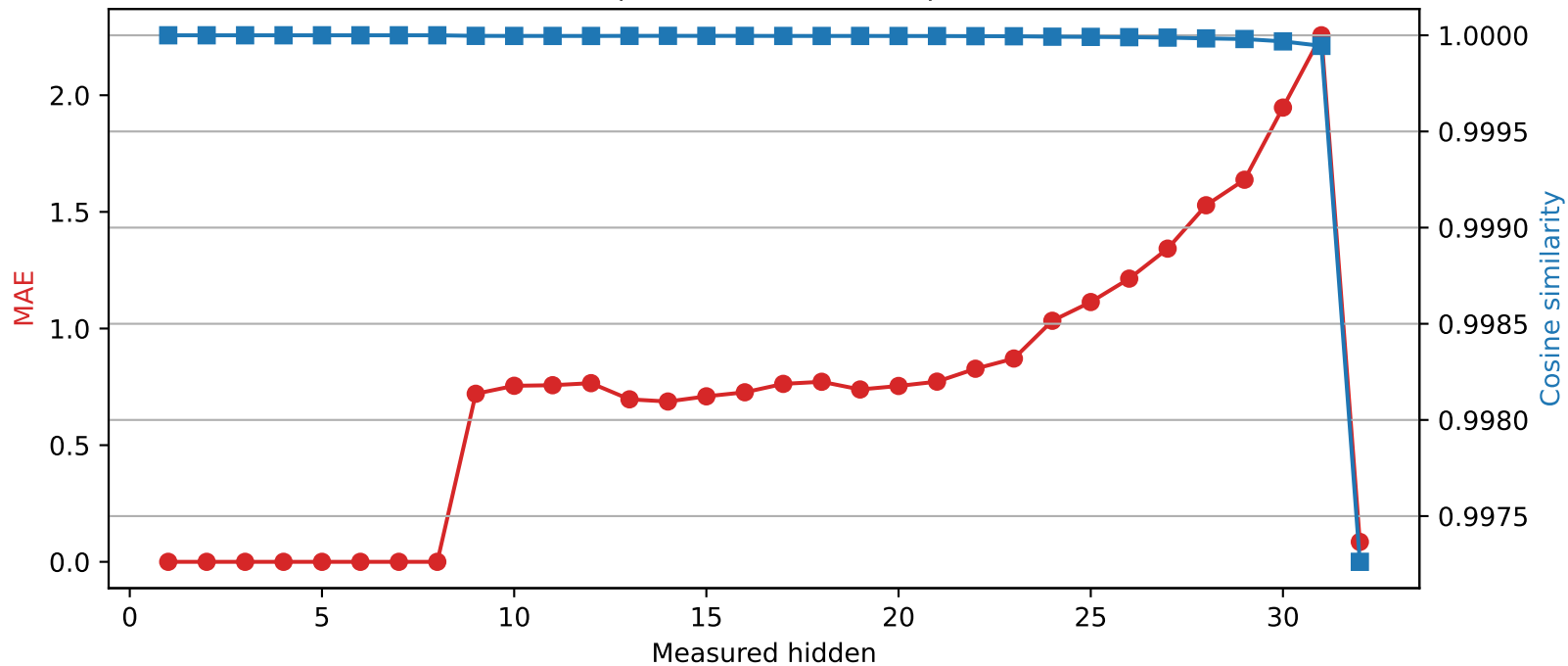
SmolLM2-360M | Quantized layer 8 | float64 → int4
