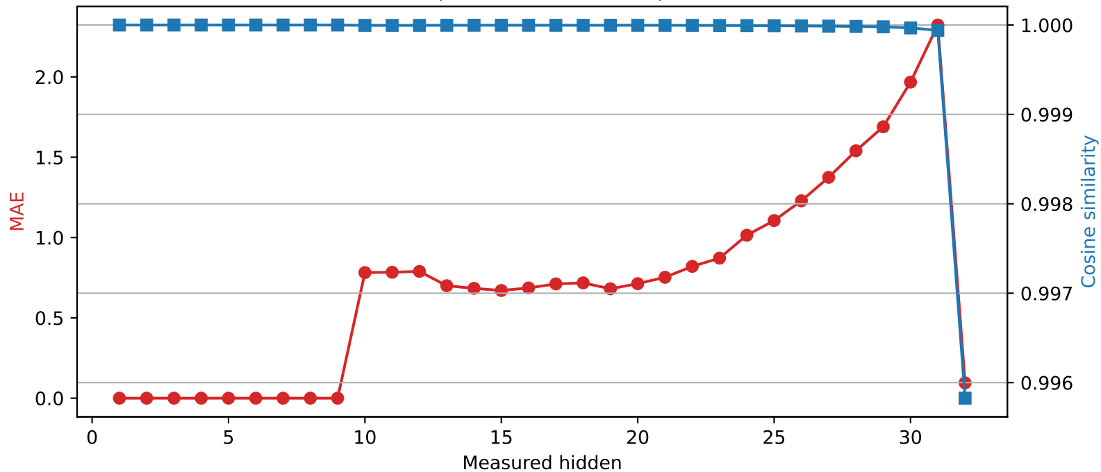
SmolLM2-360M | Quantized layer 9 | float64 → int4
