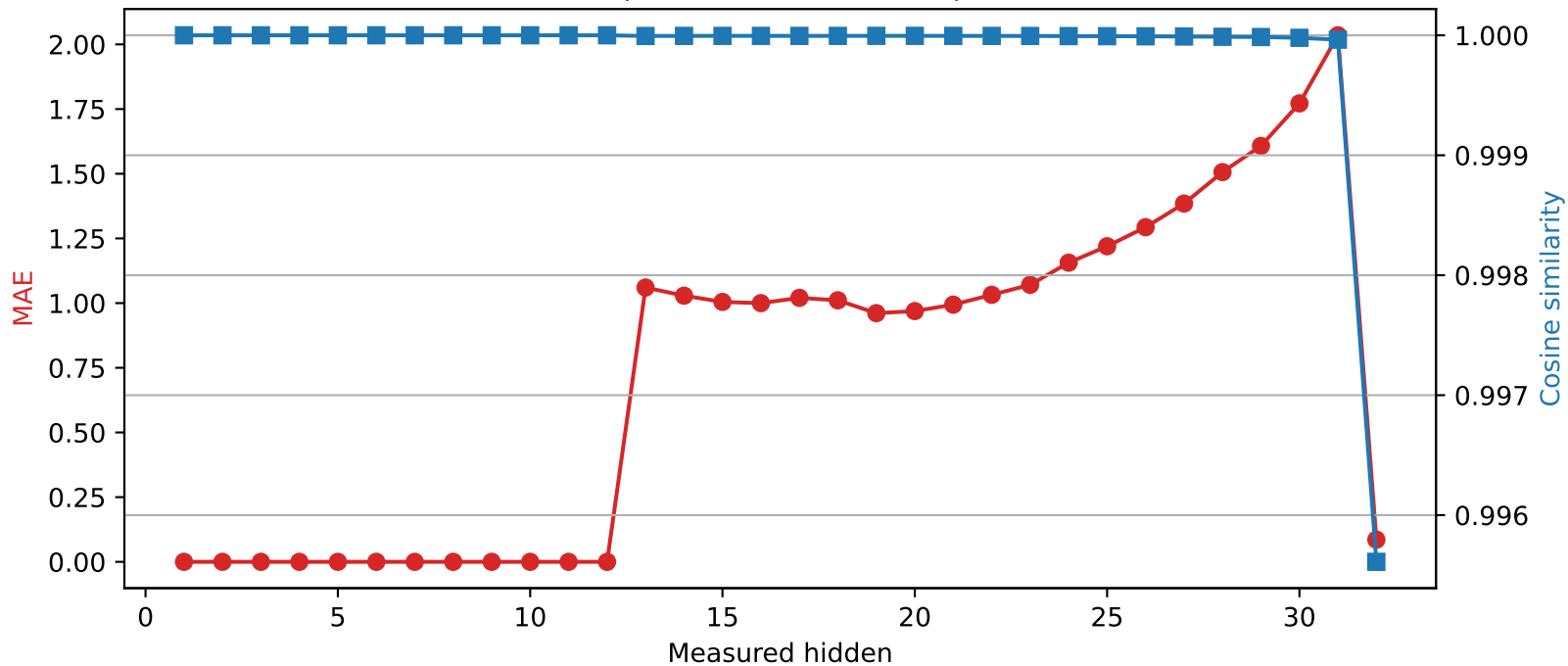
SmolLM2-360M | Quantized layer 12 | float64 → int4
