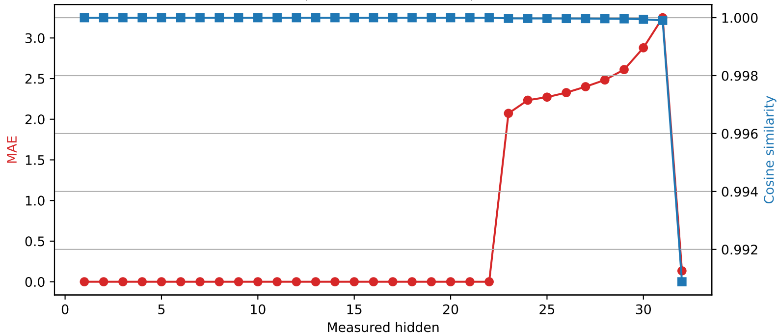
SmolLM2-360M | Quantized layer 22 | float64 → int4
