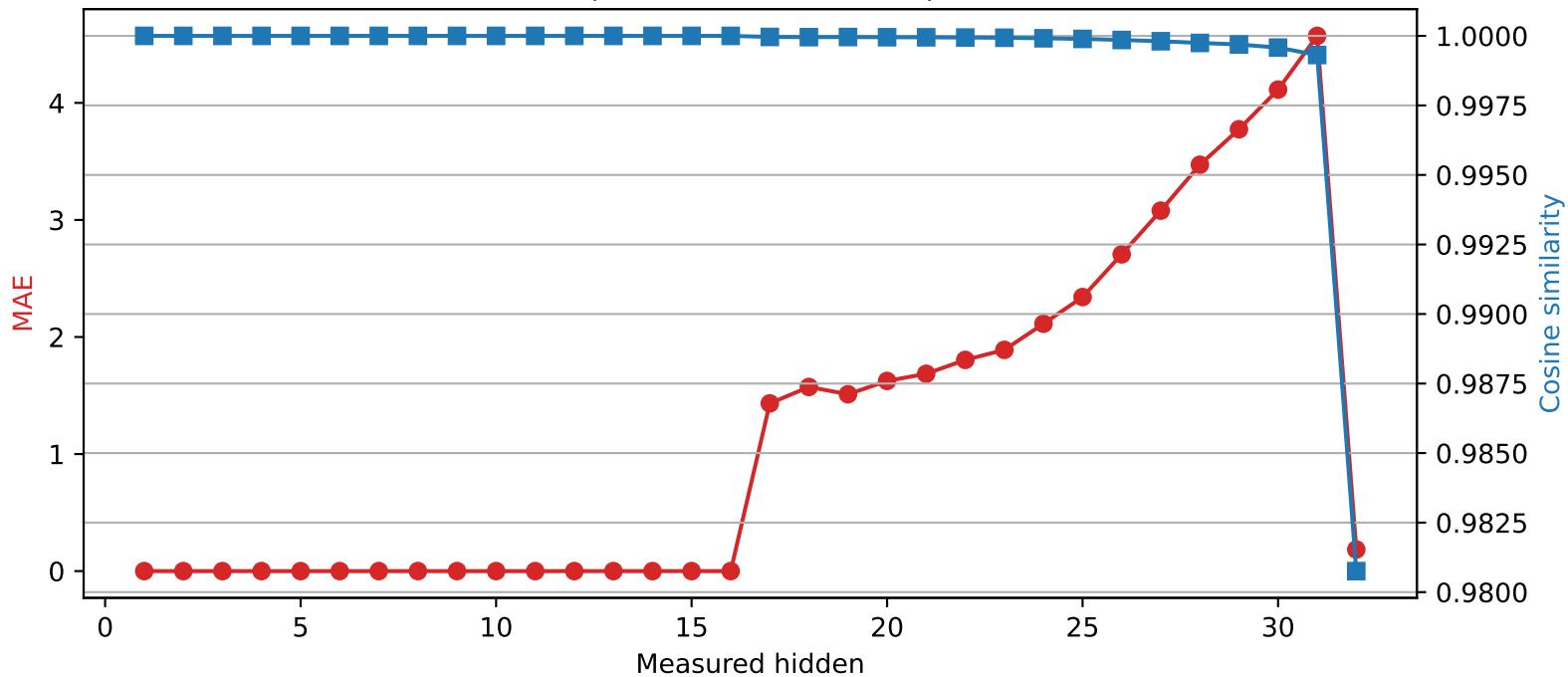
SmolLM2-360M | Quantized layer 16 | float64 → int4
