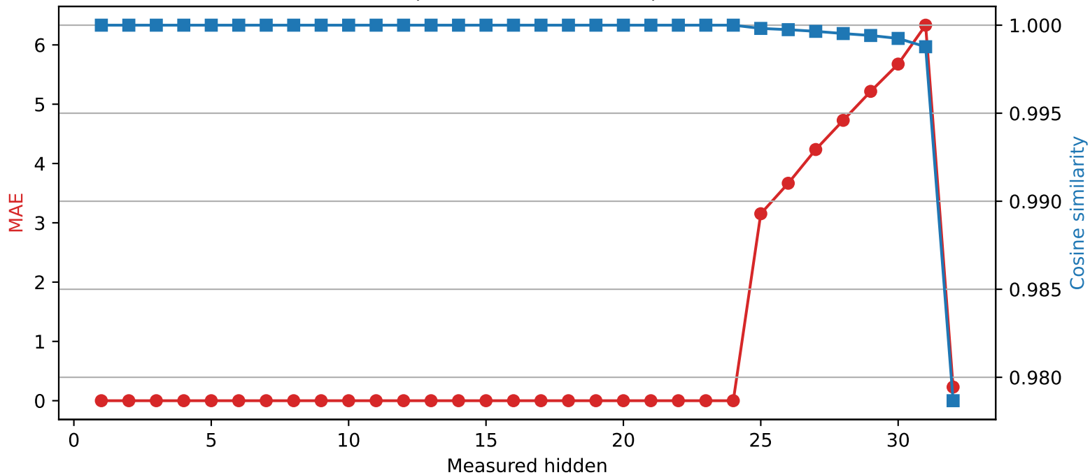
SmolLM2-360M | Quantized layer 24 | float64 → int4
