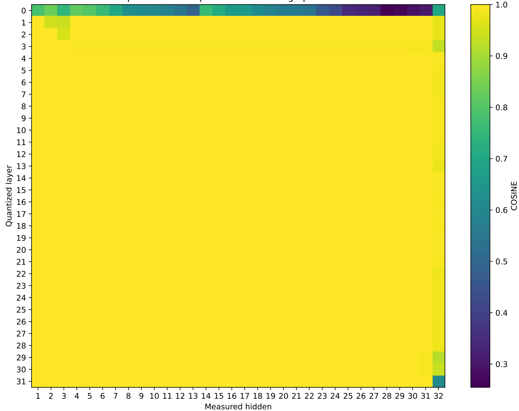
SmolLM2-360M Prompt 2: cos sim representation damage | float64 → int4
