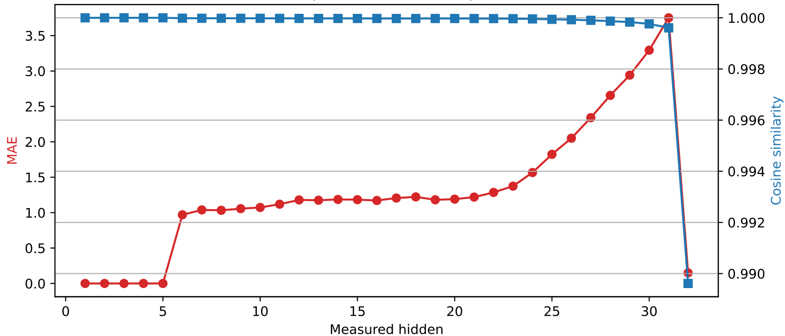
SmolLM2-360M | Quantized layer 5 | float64 → int4
