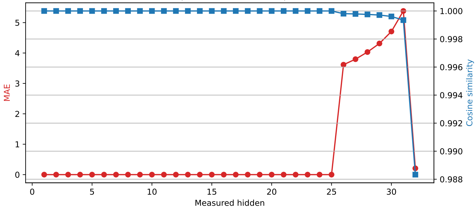
SmolLM2-360M | Quantized layer 25 | float64 → int4
