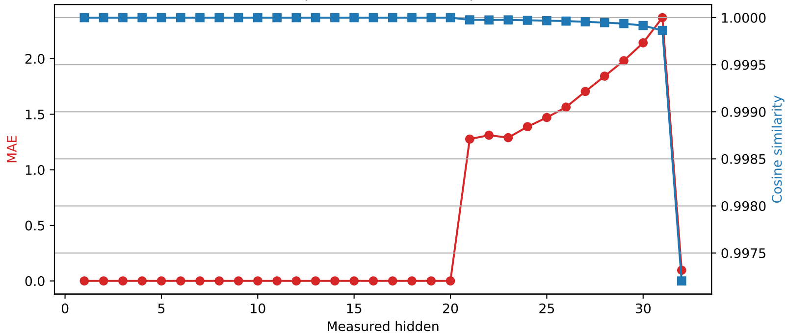
SmolLM2-360M | Quantized layer 20 | float64 → int4
