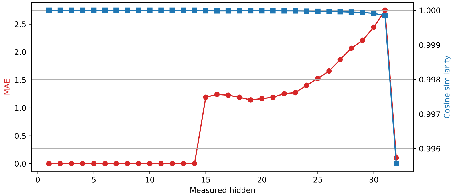
SmolLM2-360M | Quantized layer 14 | float64 → int4
