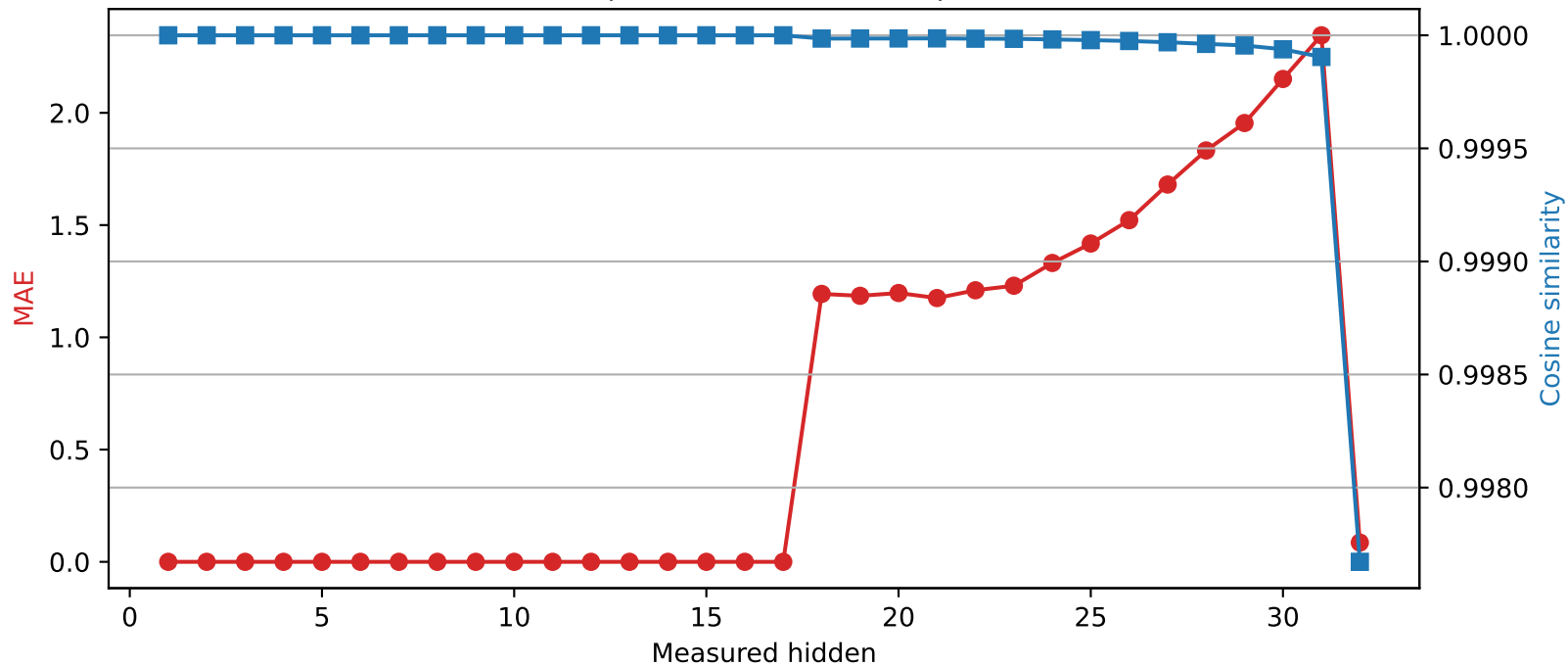
SmolLM2-360M | Quantized layer 17 | float64 → int4
