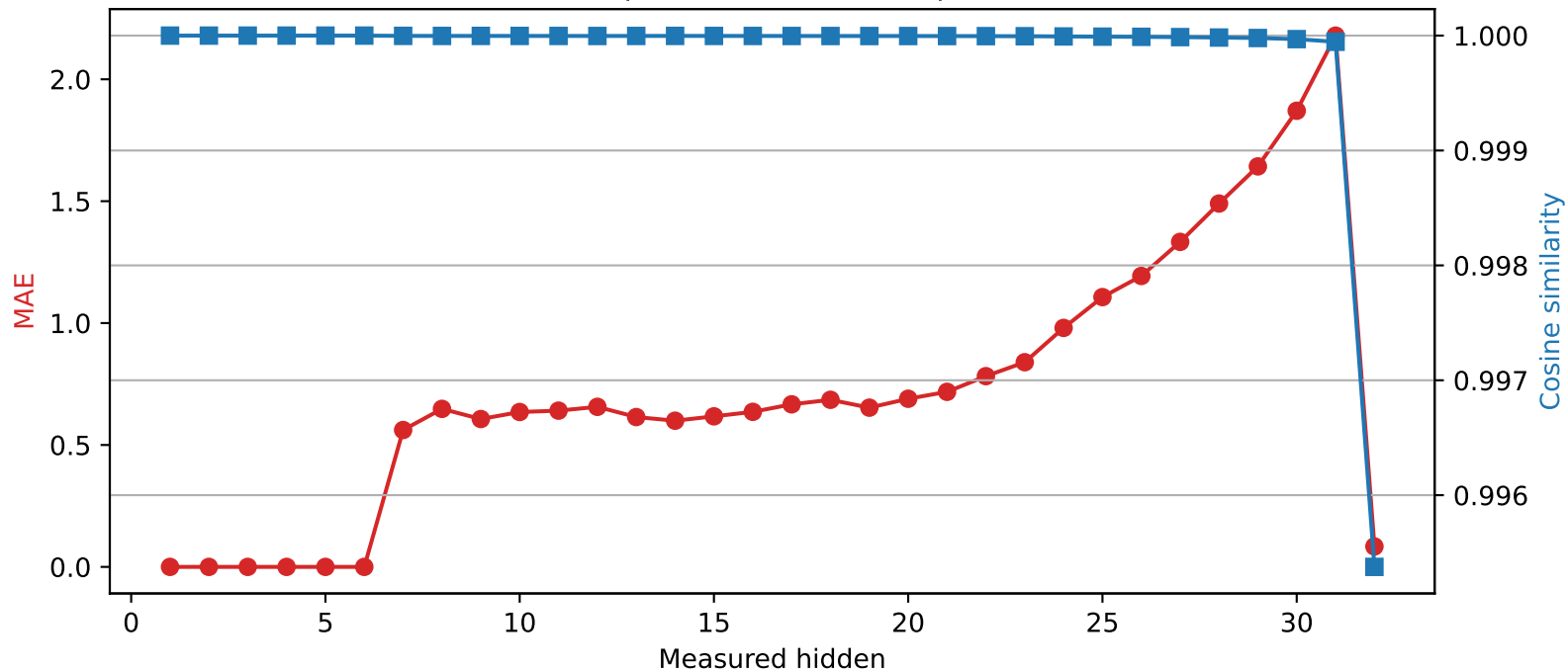
SmolLM2-360M | Quantized layer 6 | float16 \rightarrow int2
