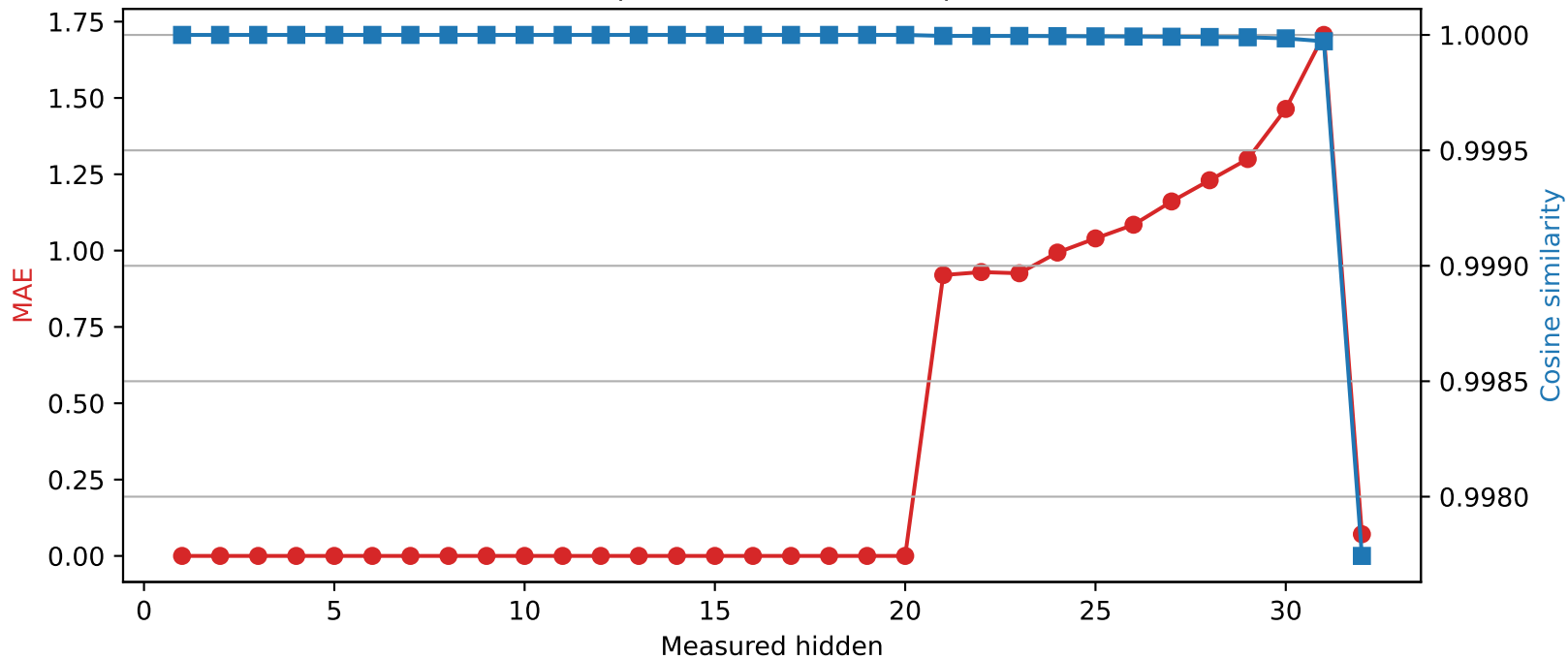
SmolLM2-360M | Quantized layer 20 | float16 \rightarrow int2
