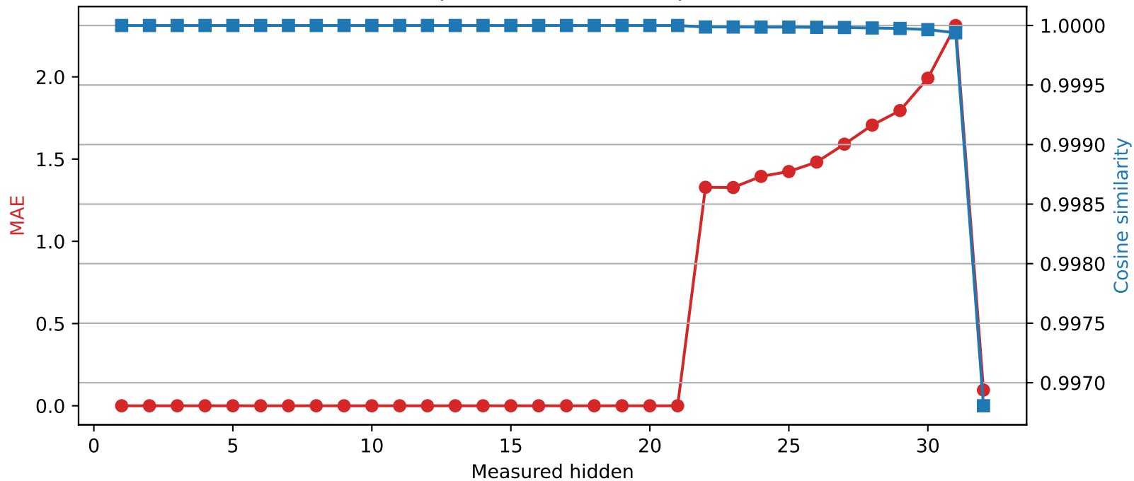
SmolLM2-360M | Quantized layer 21 | float16 \rightarrow int2
