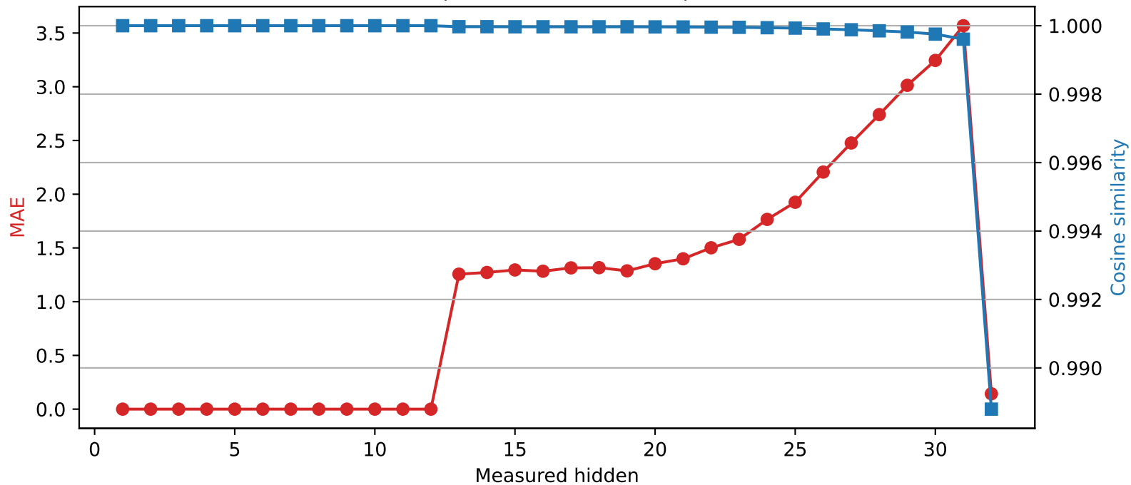
SmolLM2-360M | Quantized layer 12 | float16 \rightarrow int2
