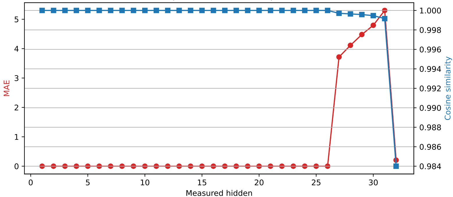
SmolLM2-360M | Quantized layer 26 | float16 → int2
