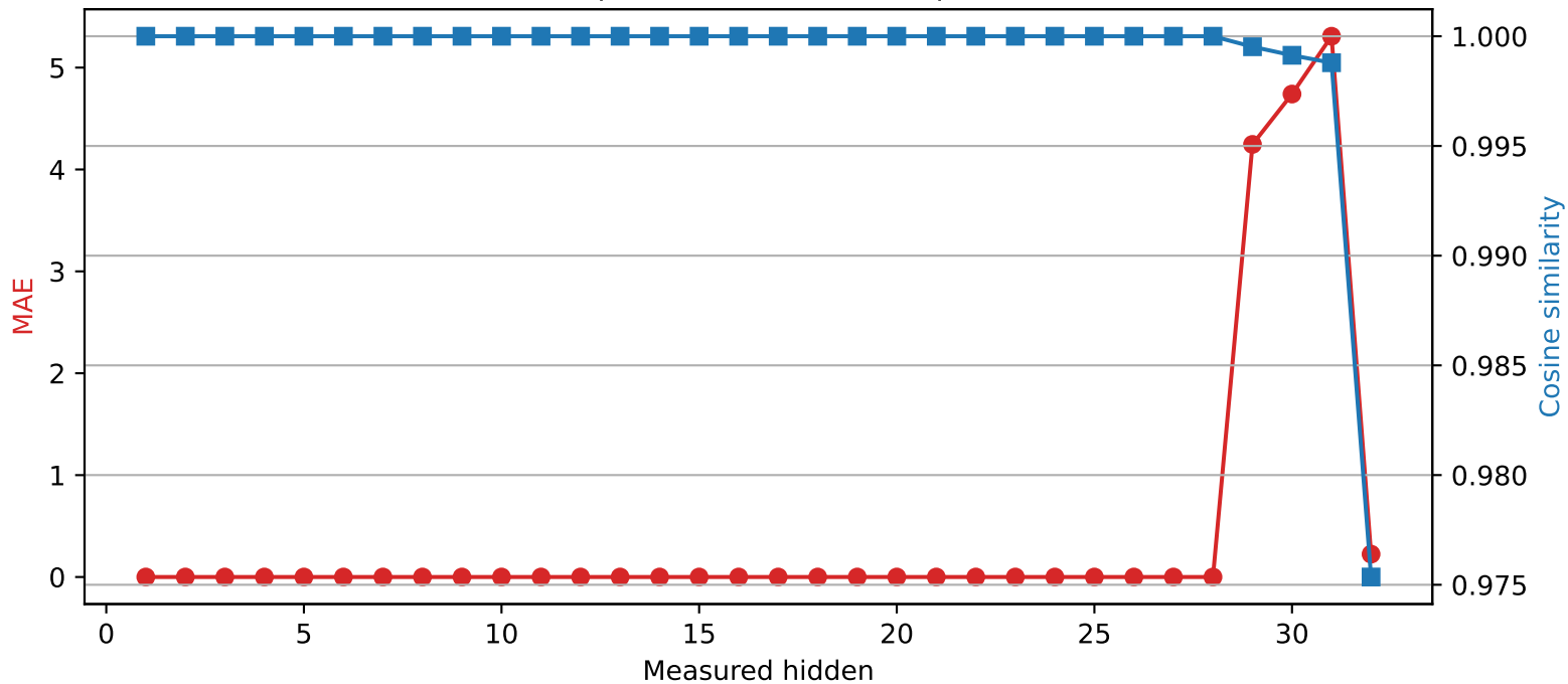
SmolLM2-360M | Quantized layer 28 | float16 \rightarrow int2
