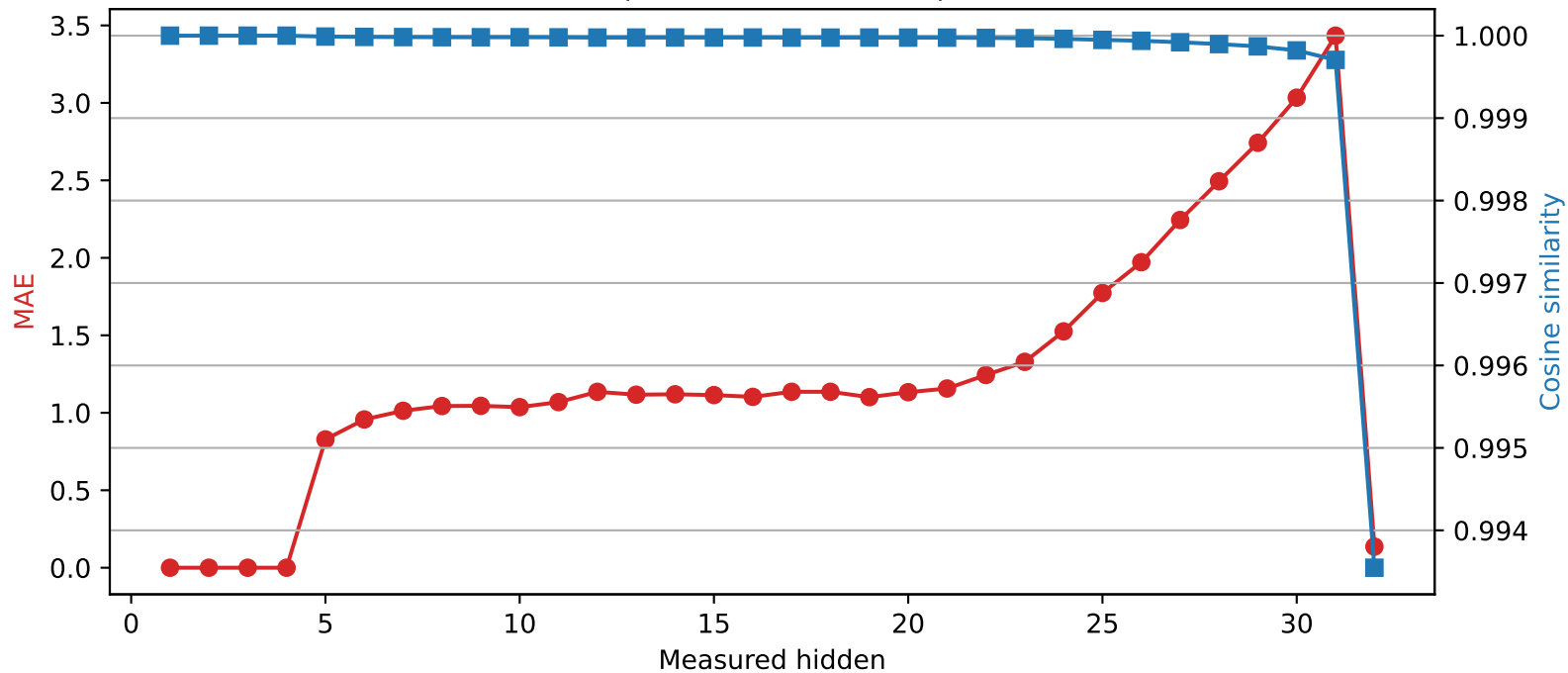
SmolLM2-360M | Quantized layer 4 | float16 \rightarrow int2
