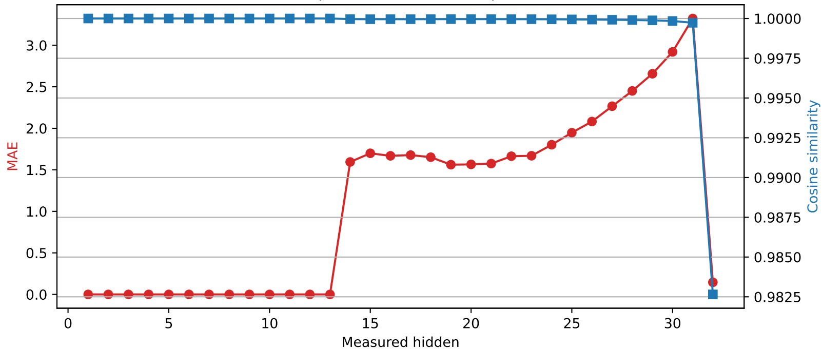
SmolLM2-360M | Quantized layer 13 | float16 \rightarrow int2
