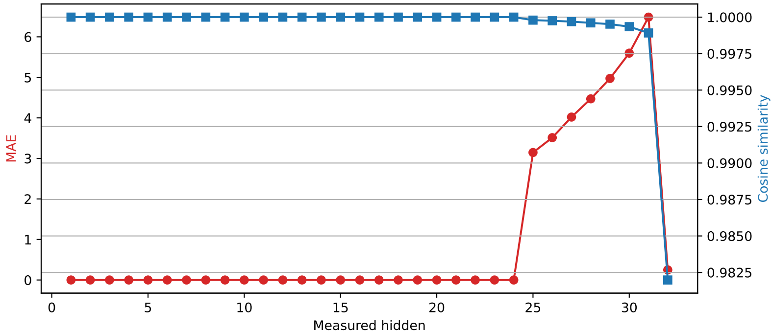
SmolLM2-360M | Quantized layer 24 | float16 → int2
