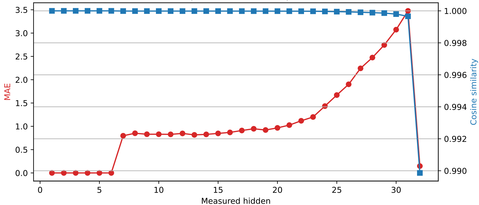
SmolLM2-360M | Quantized layer 6 | float16 → int2
