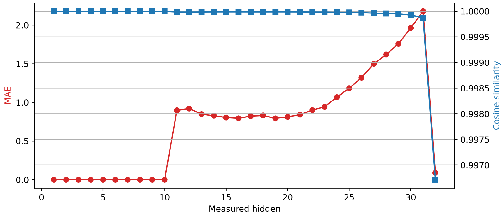
SmolLM2-360M | Quantized layer 10 | float16 \rightarrow int2
